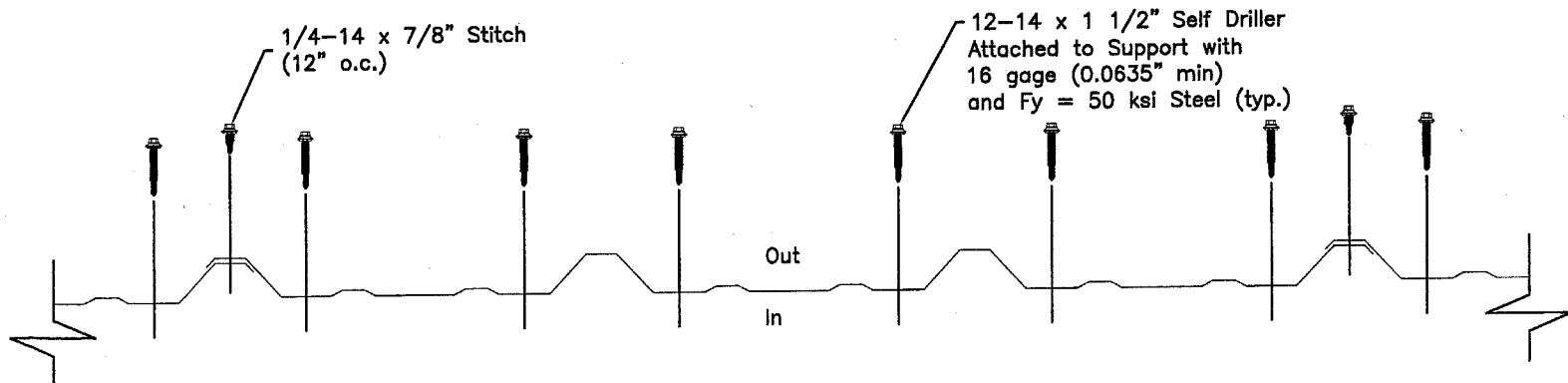
R-Panel Fastening Pattern (Ends & Endlap Splice)
