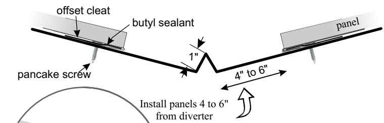
Fig. 20 Lap detail for offset cleat on transition flashing or valley.
