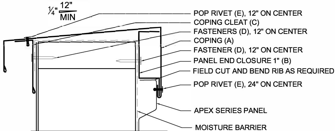
ELEVATION VIEW
