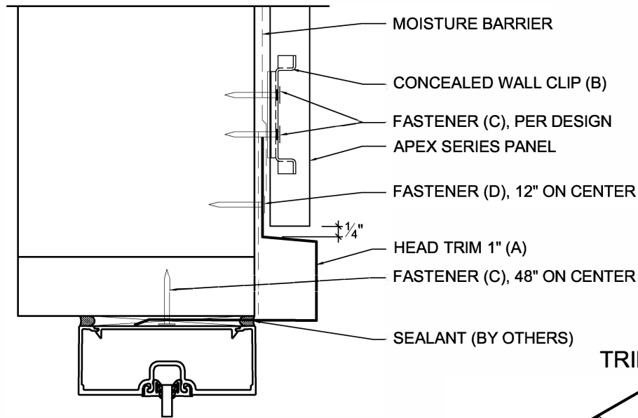
ELEVATION VIEW
