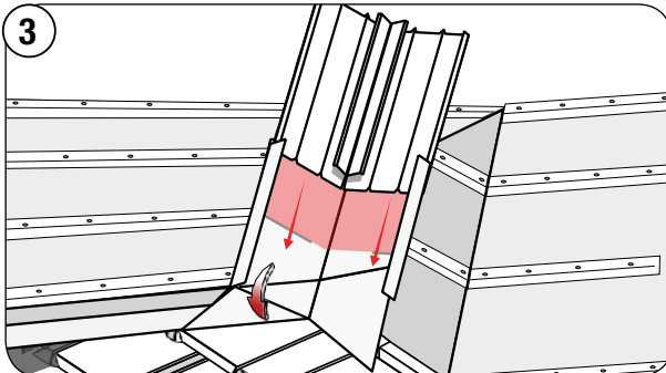
Install Valley metal over and onto the stone coated Flat Sheet. Apply a bead of sealant across the top of the Flat Sheet and embed the Valley into the sealant.
