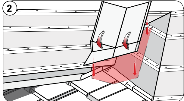
Form the stone coated Flat Sheet as an extension and exit tray for the upcoming valley. Apply sealant under the Flat Sheet where it exits on top of the panel beneath.
