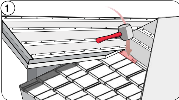
Flatten back flange against the roof deck.
