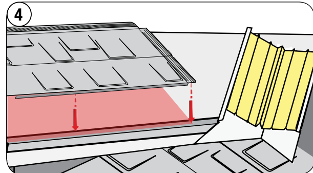
Then install the panels regularly as valley cut sections into the Valley 2-Pc.
