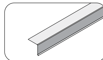
Drip Edge 1.5" x 120" (38 x 3048 mm) 1.6 lbs (0.72 Kg) Painted Black, Brown or White outside
