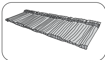
PINE-CREST Shake Panel Coverage: 14.5" x 49.5" (368 x 1257 mm) 6.4 lbs (2.91 Kgs) 20 pcs/sq
