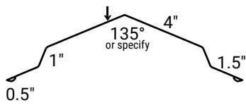
12" Ridge
