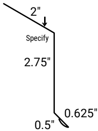
Denver Eave
