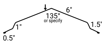
16" Ridge
