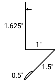
Rat Guard
