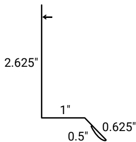
Drip Cap
