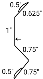
Counter Flashing
