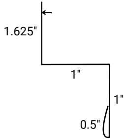
Double Angle
