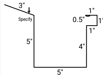
Box Gutter
